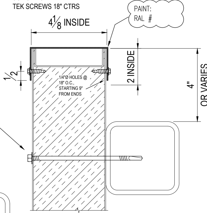
CC1- CAP CHANNEL 18 GA GALVANNEALED X 144" LG
