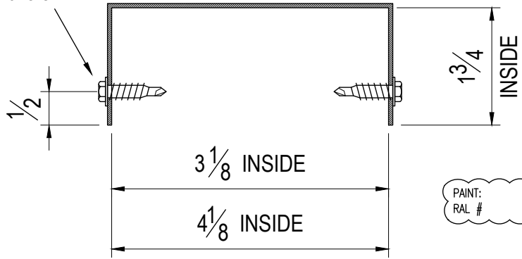
CC1- CAP CHANNEL 18 GA GALVANNEALED X 144" LG
