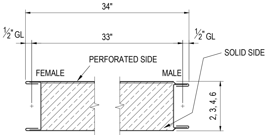
STD WIDTH UNENGAGED PANEL
