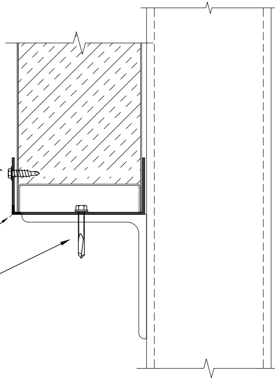
BOTTOM CHANNEL DETAIL
