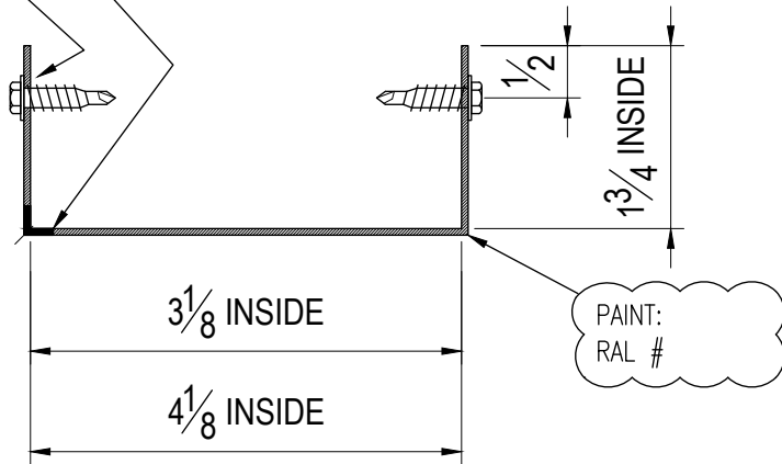
FC1- BOTTOM CHANNEL 18 GA GALVANNEALED X 144" LG
